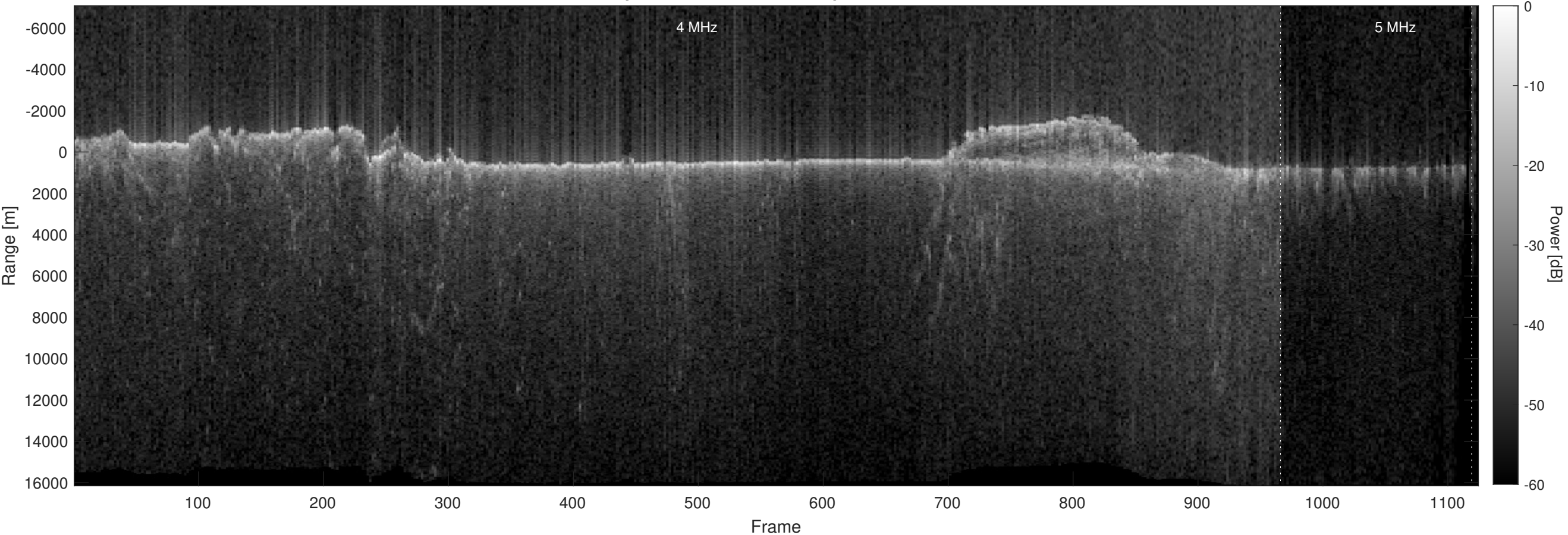
Orbit 12007, Optimized, No Window, Depth-Corrected, Channel 2
