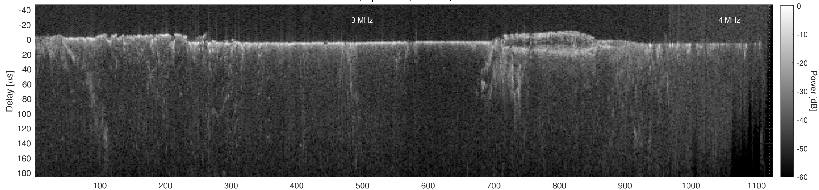
Orbit 12007, Cluttergram
