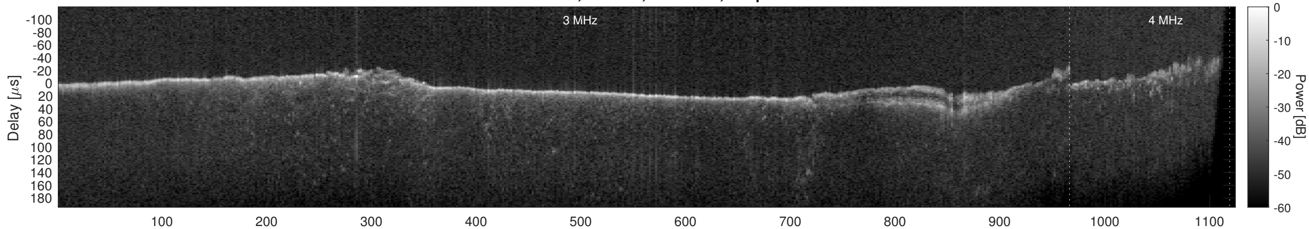
Orbit 12008, Window, Channel 2, Optimized
