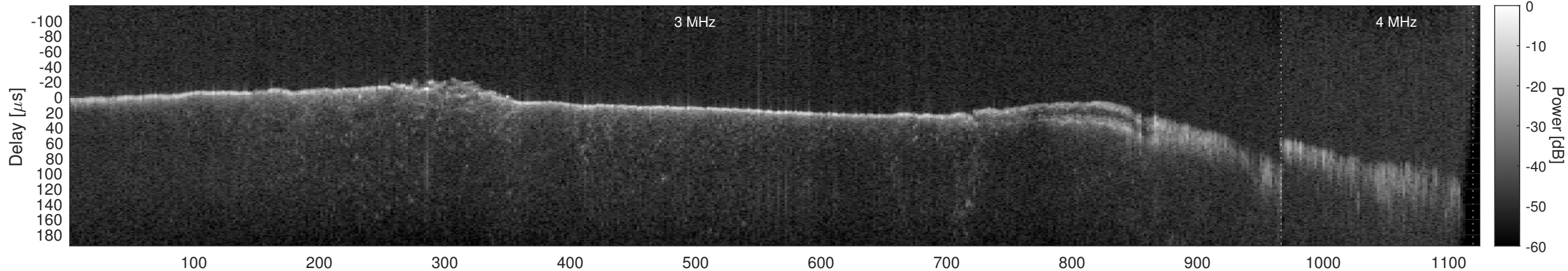
Orbit 12008, Window, Channel 2, Chapman
