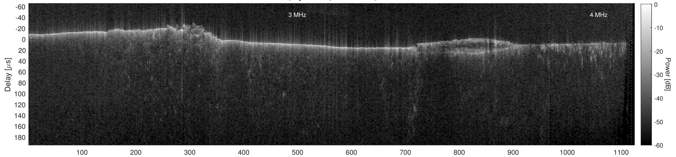
Orbit 12008, Cluttergram
