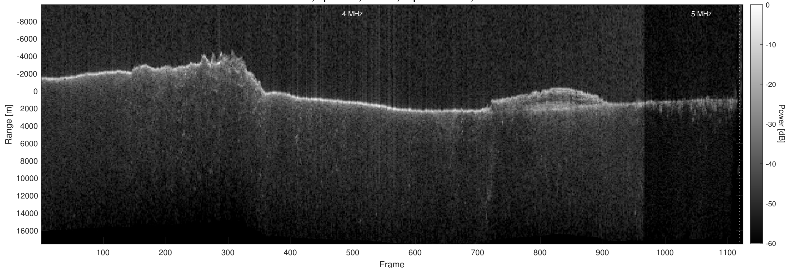
Orbit 12008, Optimized, Window, Depth-Corrected, Channel 2
