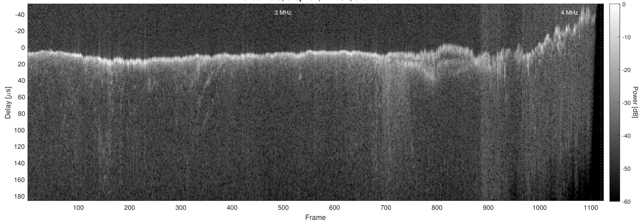
Orbit 12009, Chapman, Window, Channel 2
