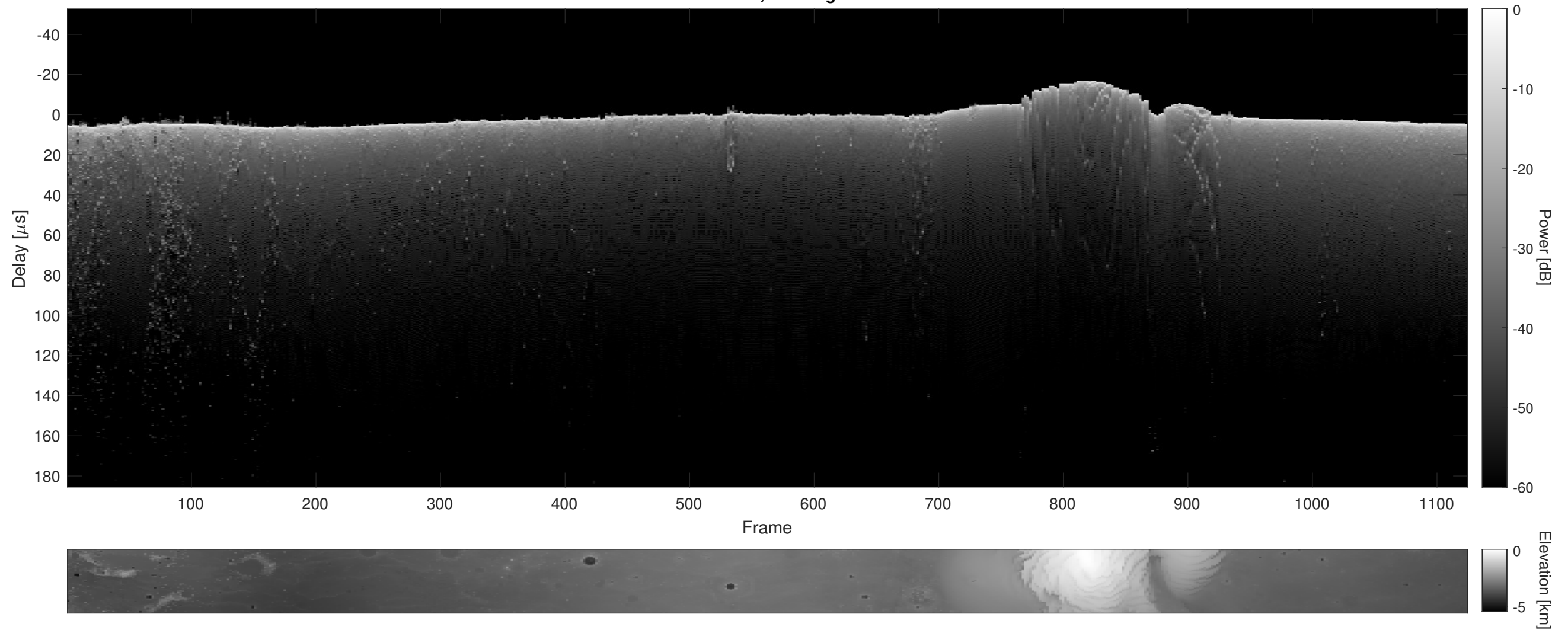
Orbit 12009, Cluttergram
