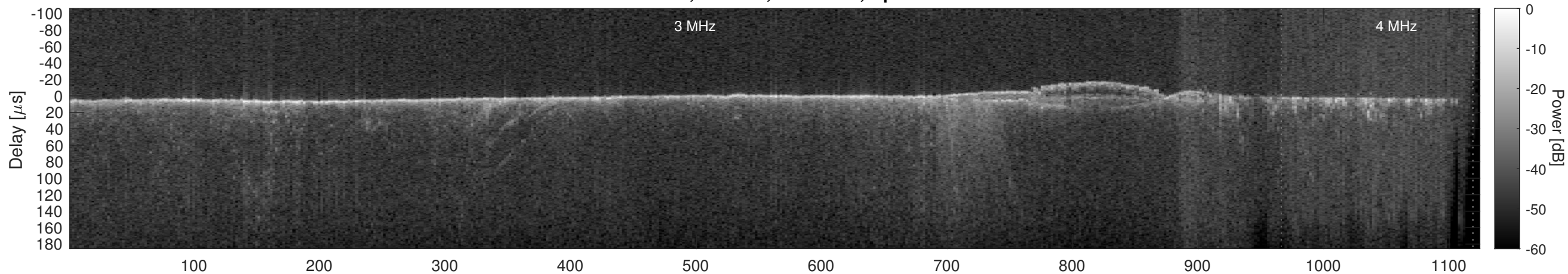
Orbit 12009, Cluttergram
