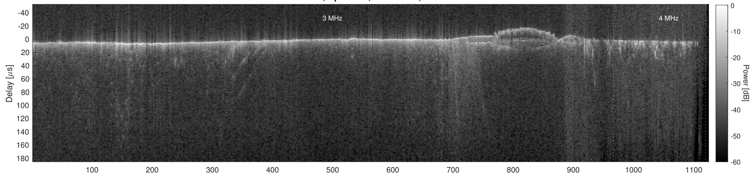
Orbit 12009, Cluttergram
