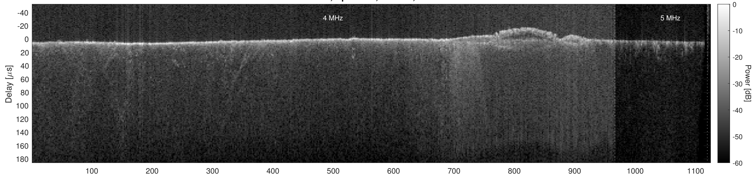
Orbit 12009, Optimized, Window, Channel 2
