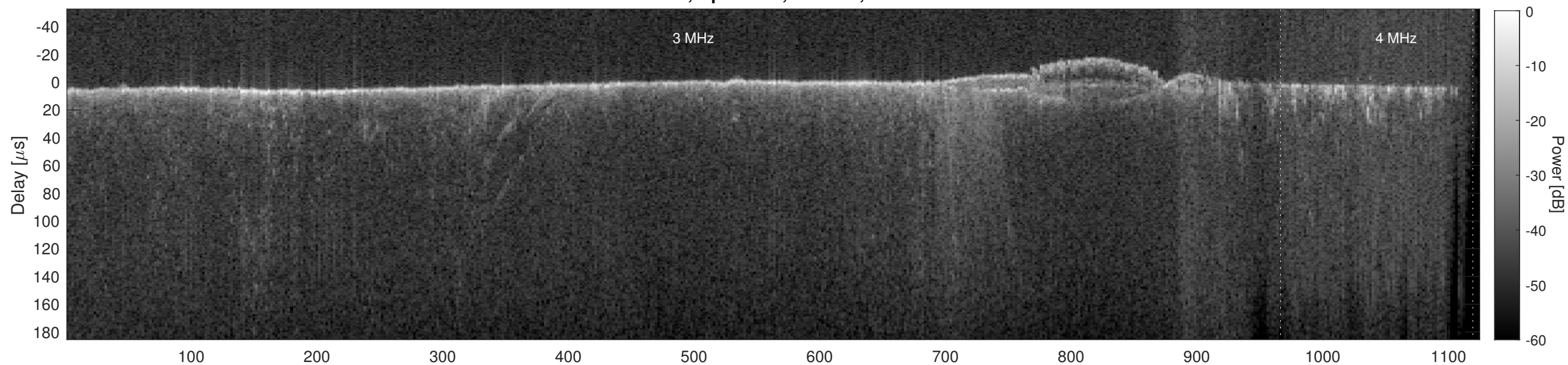
Orbit 12009, Cluttergram
