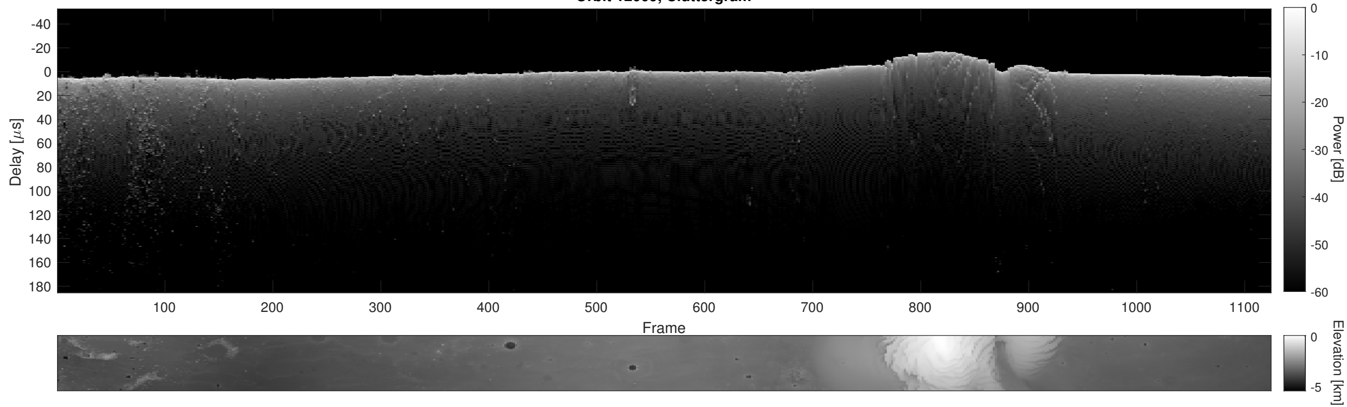
Orbit 12009, Cluttergram
