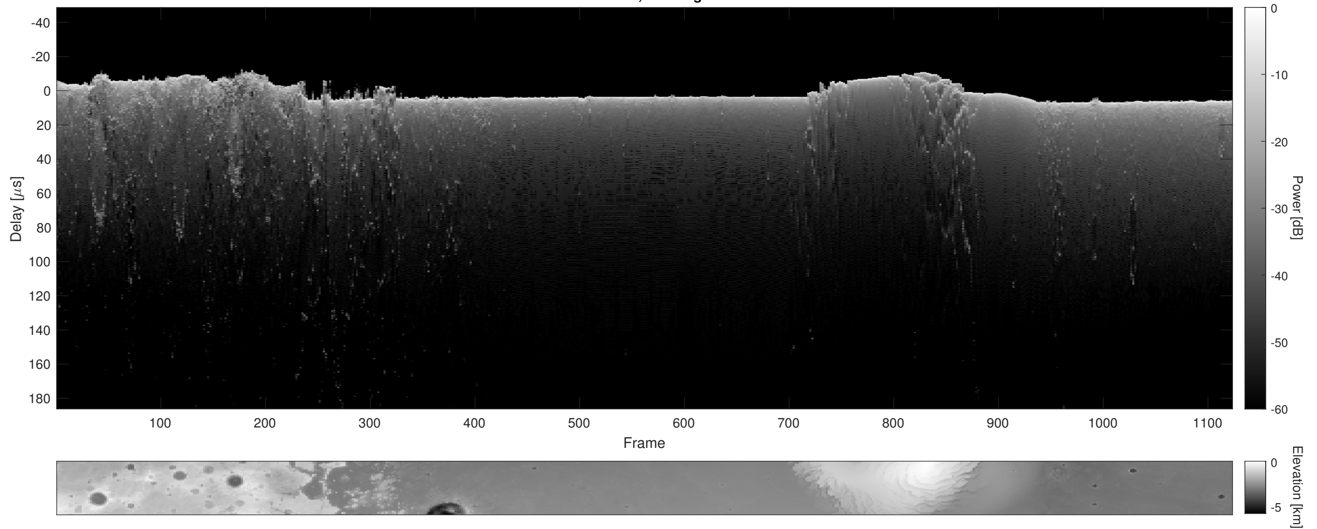
Orbit 12014, Cluttergram
