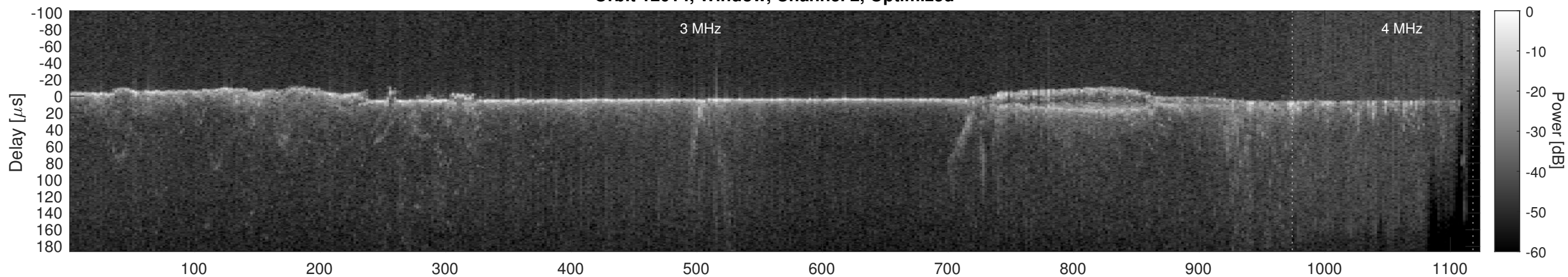
Orbit 12014, Cluttergram
