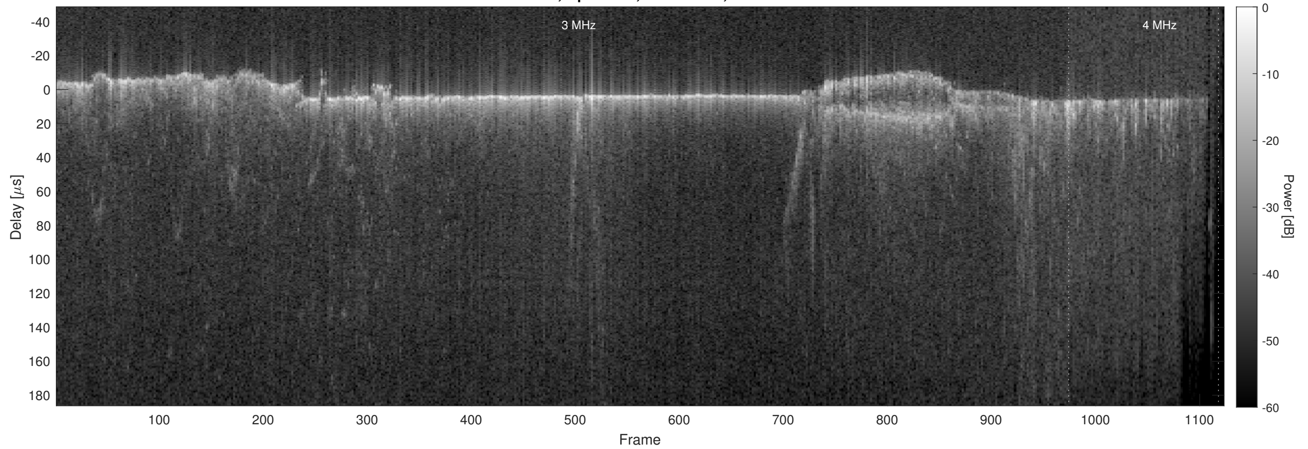
Orbit 12014, Optimized, No Window, Channel 2
