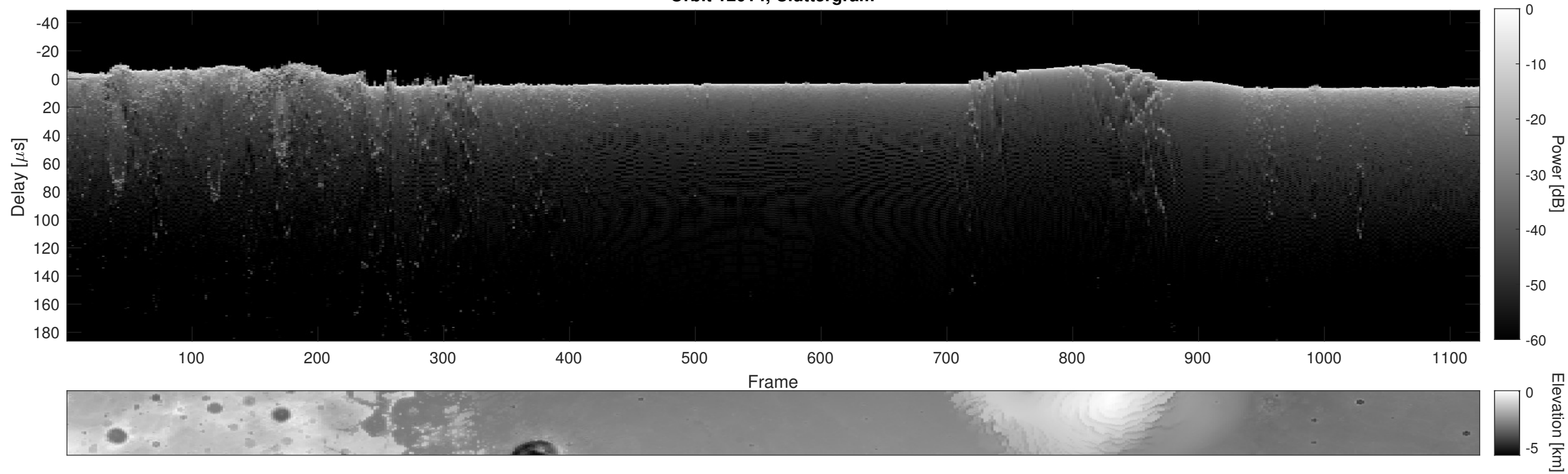
Orbit 12014, Cluttergram
