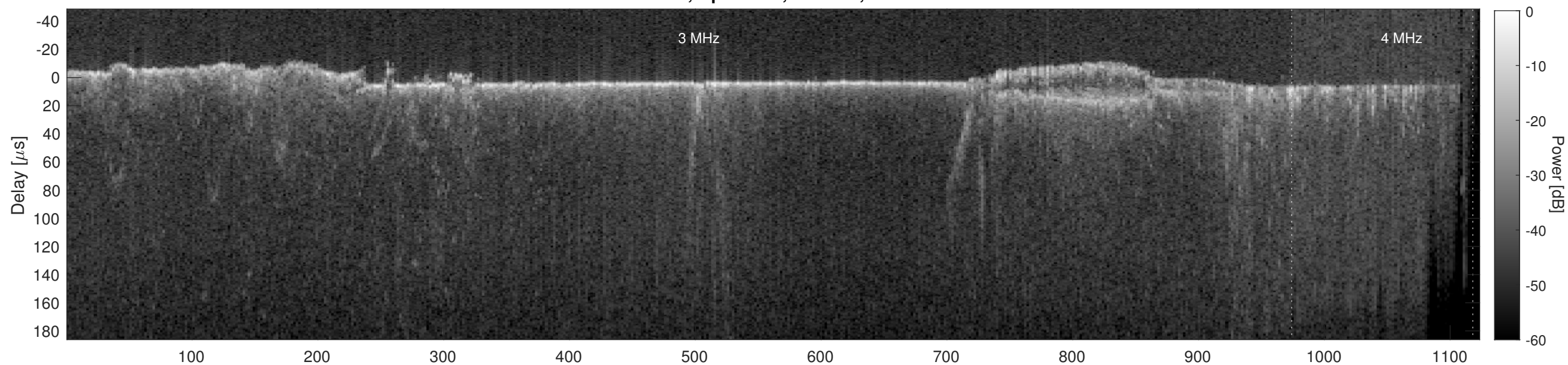
Orbit 12014, Cluttergram
