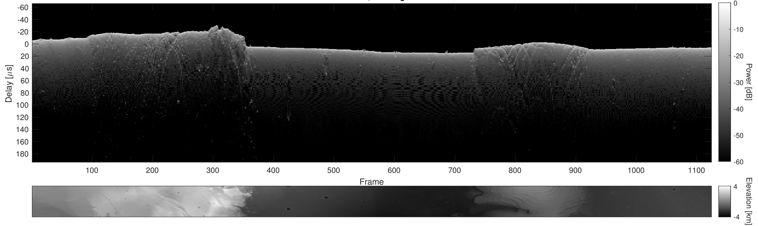
Orbit 12015, Cluttergram
