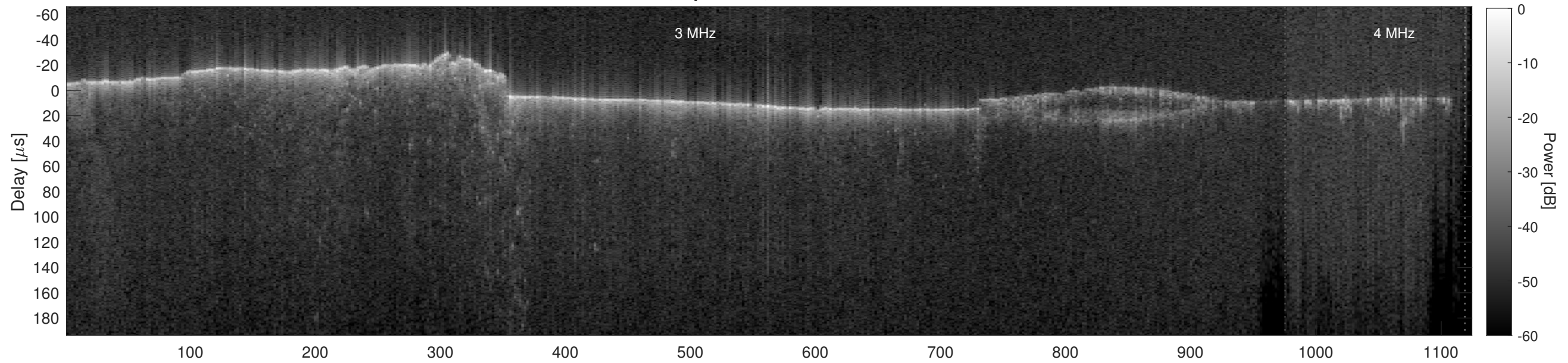
Orbit 12015, Cluttergram
