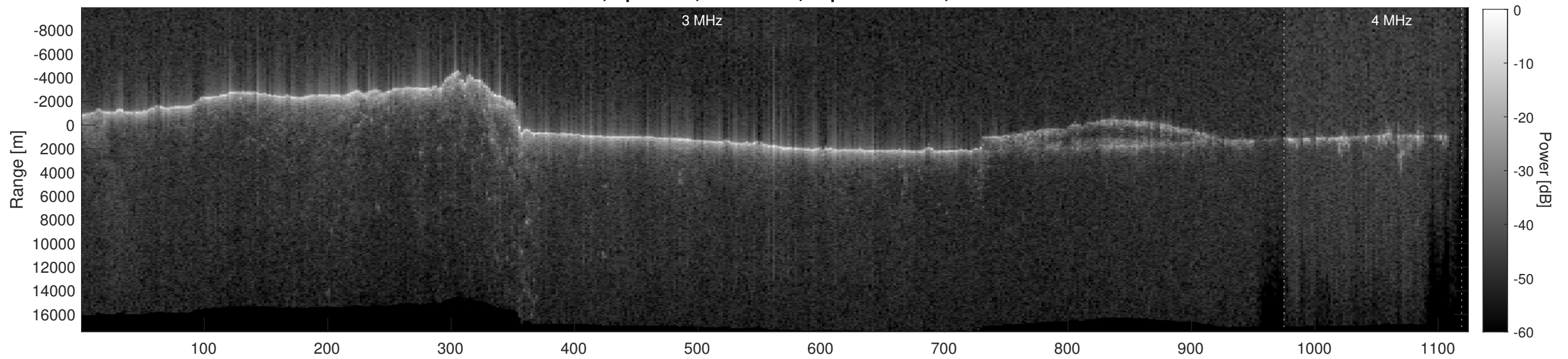
Orbit 12015, Depth-Corrected Cluttergram
