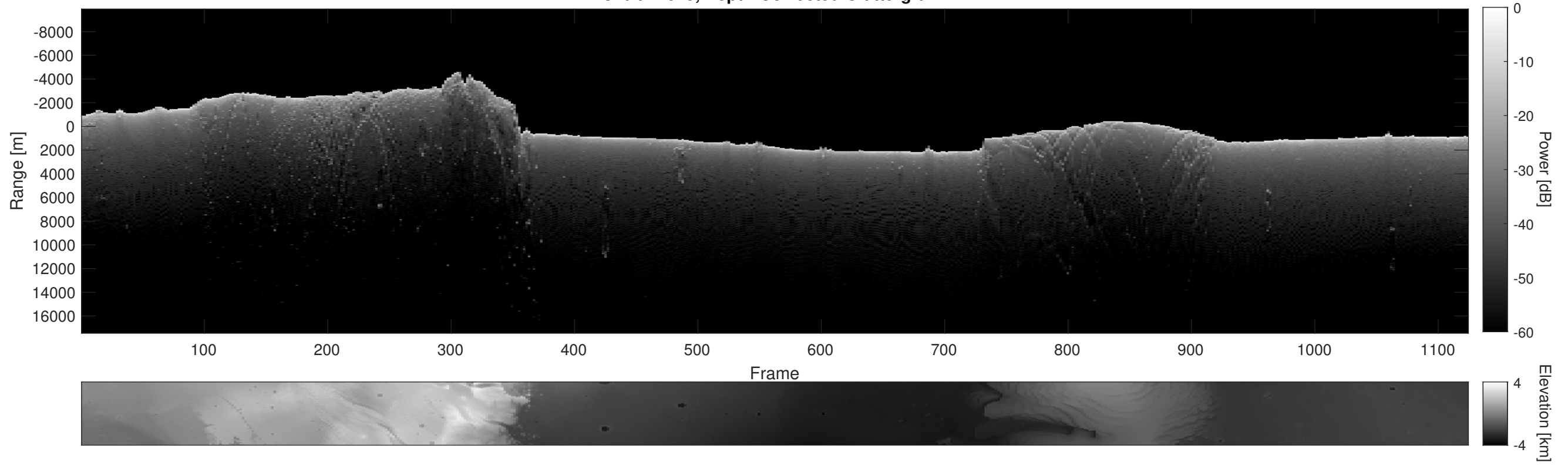
Orbit 12015, Depth-Corrected Cluttergram
