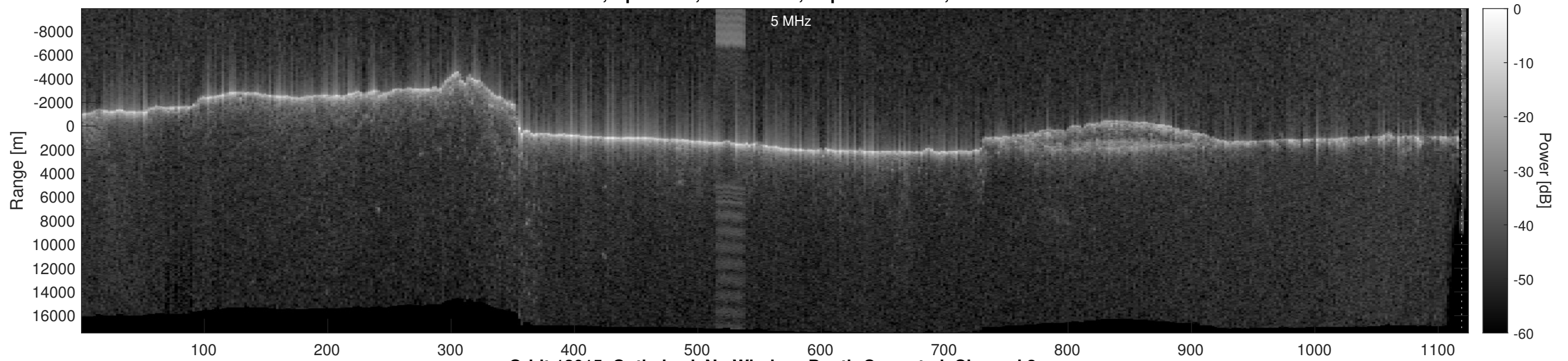
Orbit 12015, Optimized, No Window, Depth-Corrected, Channel 2
