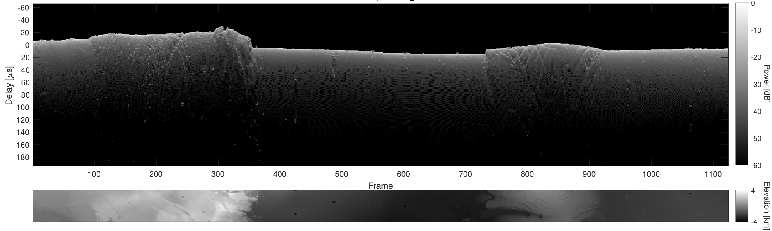
Orbit 12015, Cluttergram
