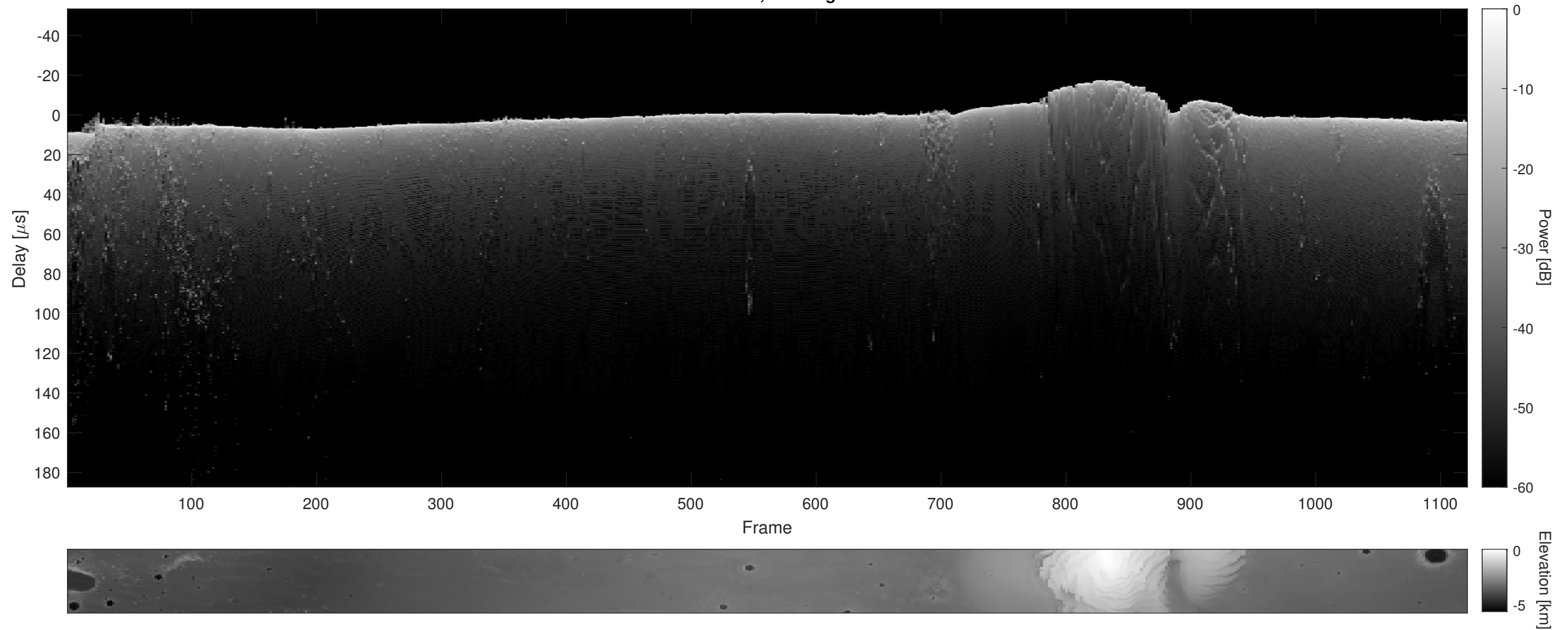
Orbit 12016, Cluttergram
