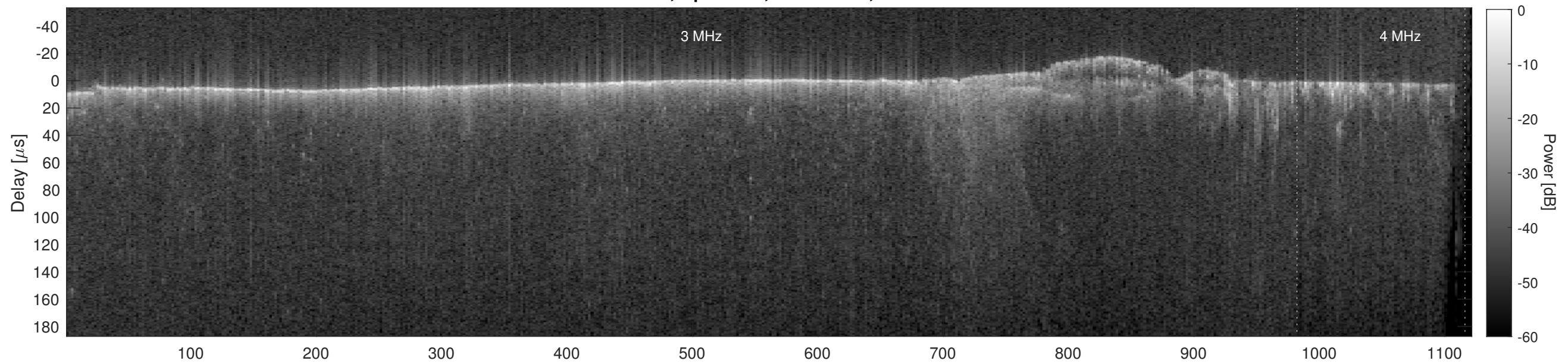
Orbit 12016, Cluttergram
