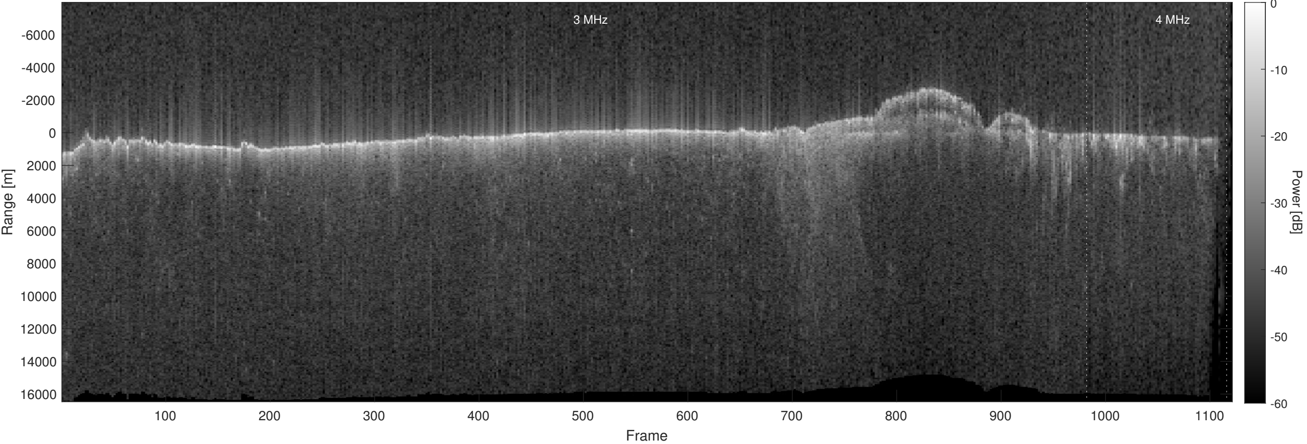
Orbit 12016, Optimized, No Window, Depth-Corrected, Channel 2
