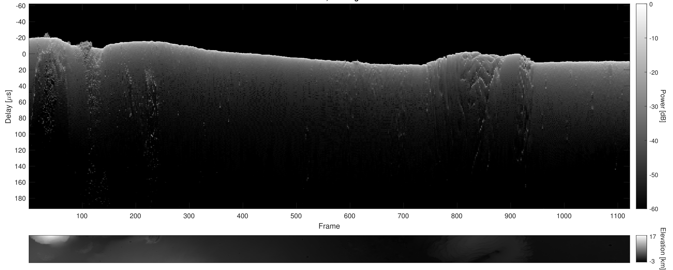
Orbit 12019, Cluttergram
