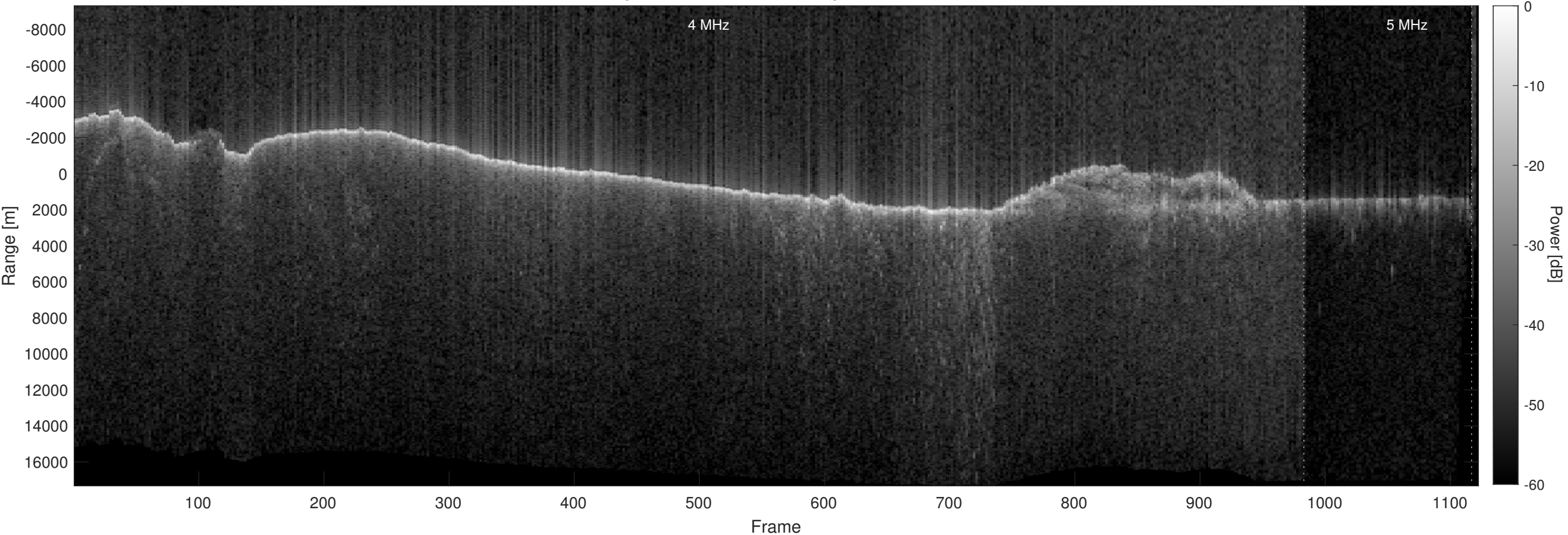
Orbit 12019, Optimized, No Window, Depth-Corrected, Channel 2
