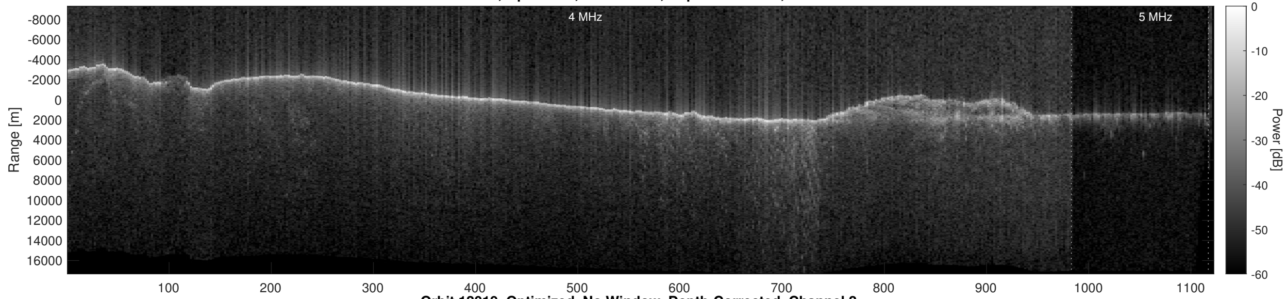
Orbit 12019, Optimized, No Window, Depth-Corrected, Channel 2
