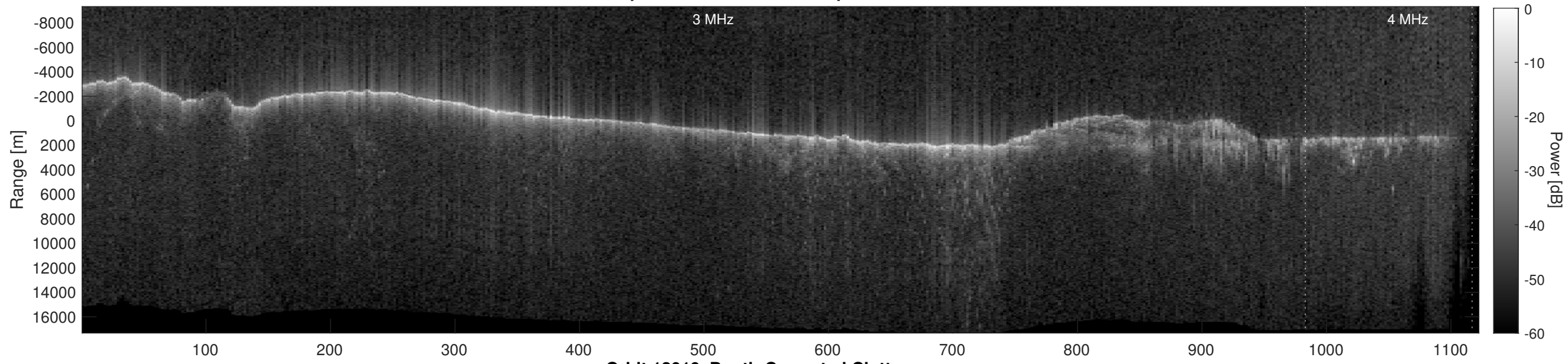
Orbit 12019, Depth-Corrected Cluttergram
