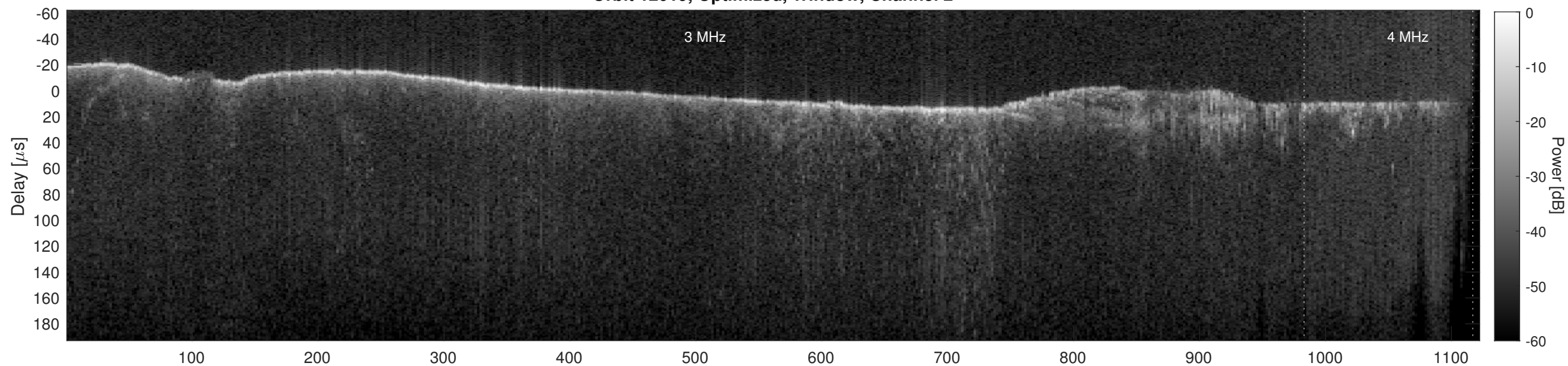
Orbit 12019, Cluttergram
