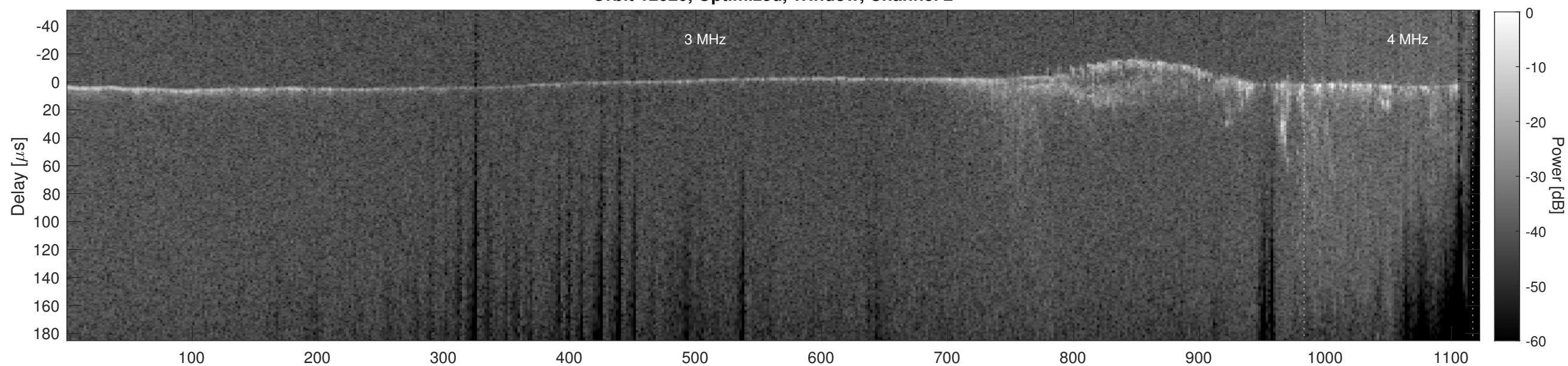
Orbit 12020, Cluttergram
