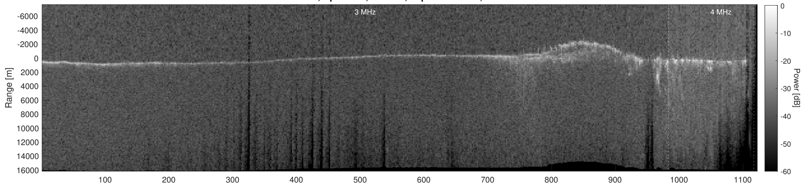
Orbit 12020, Depth-Corrected Cluttergram
