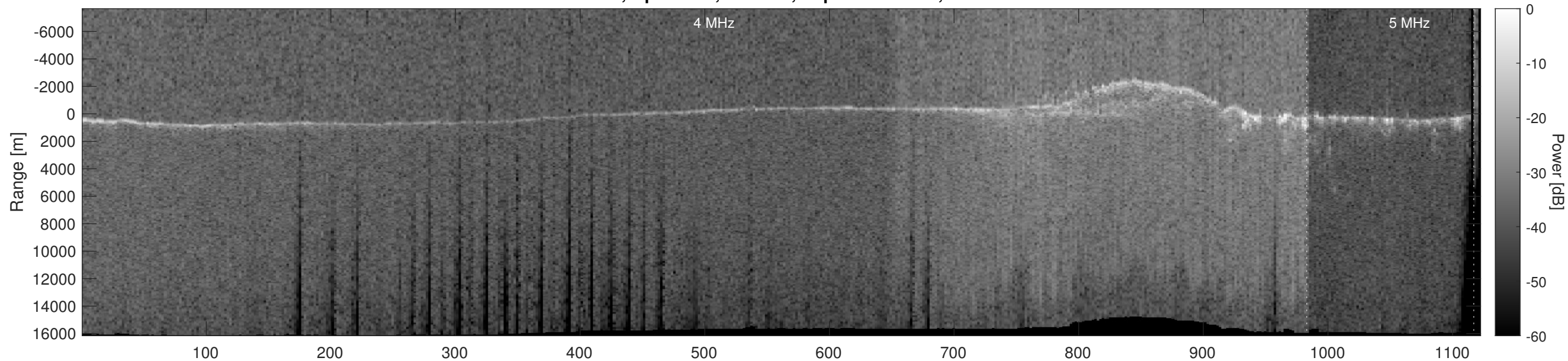
Orbit 12020, Optimized, Window, Depth-Corrected, Channel 2
