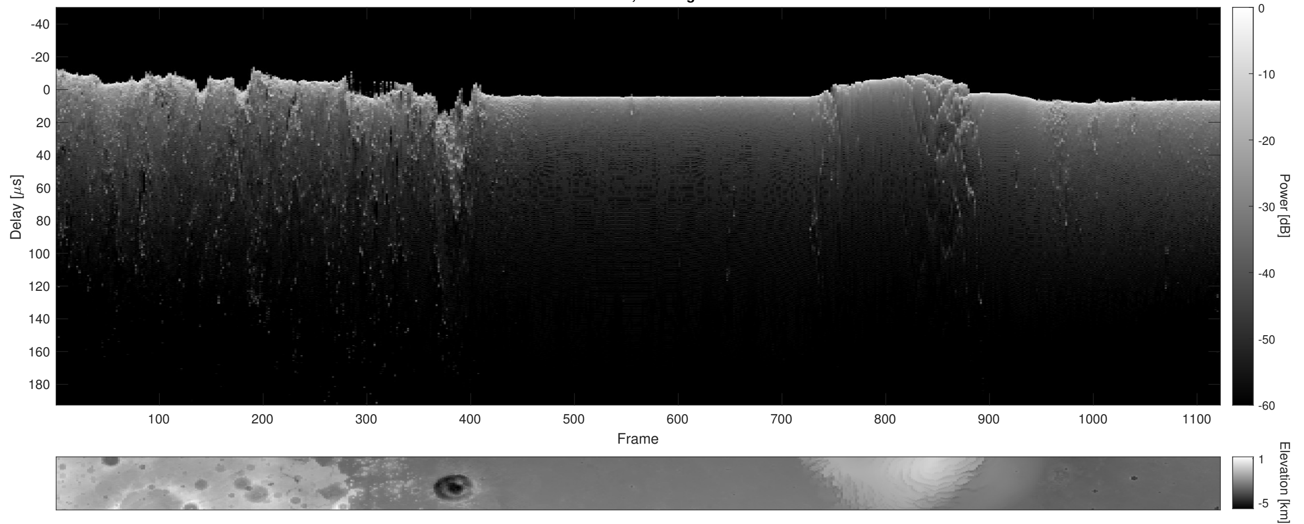
Orbit 12021, Cluttergram
