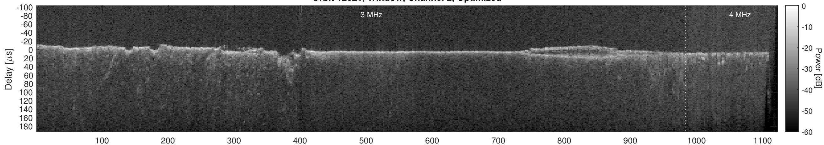
Orbit 12021, Cluttergram
