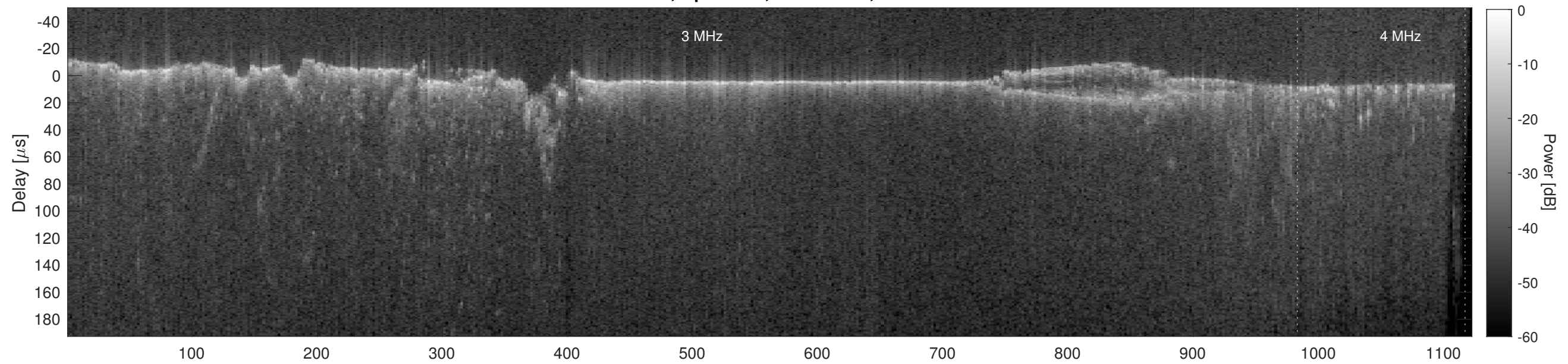
Orbit 12021, Cluttergram
