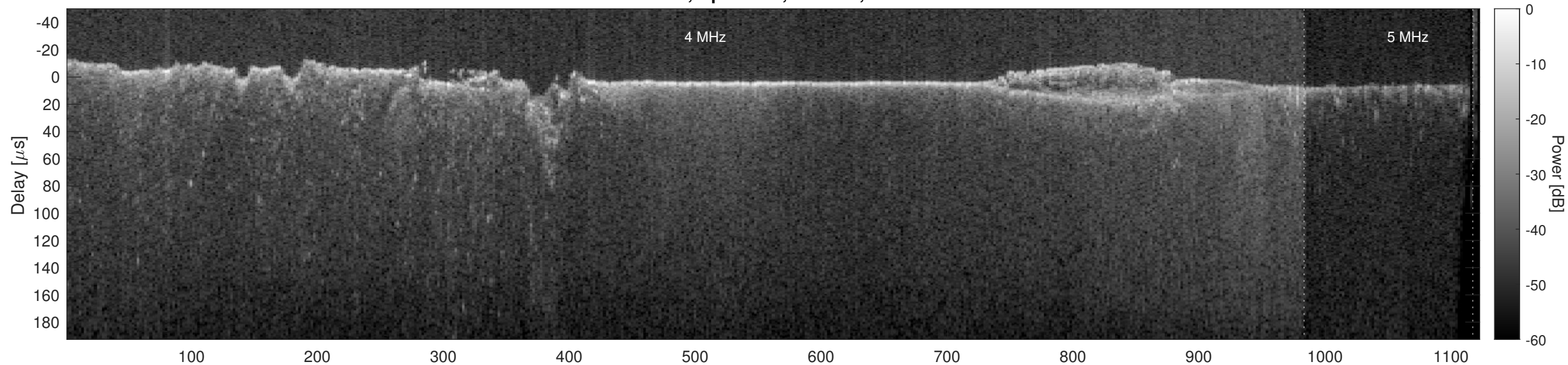
Orbit 12021, Optimized, Window, Channel 2
