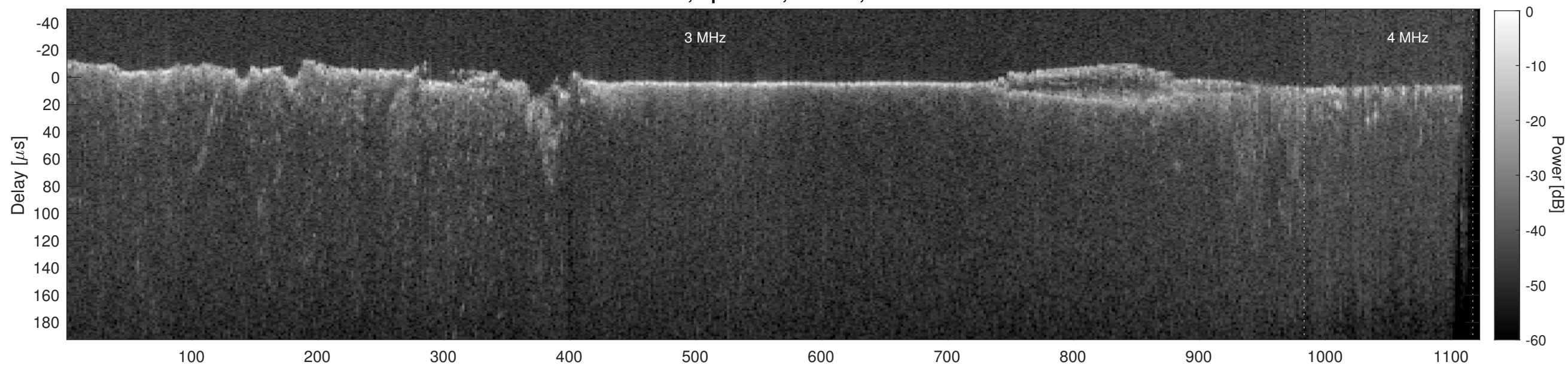
Orbit 12021, Cluttergram
