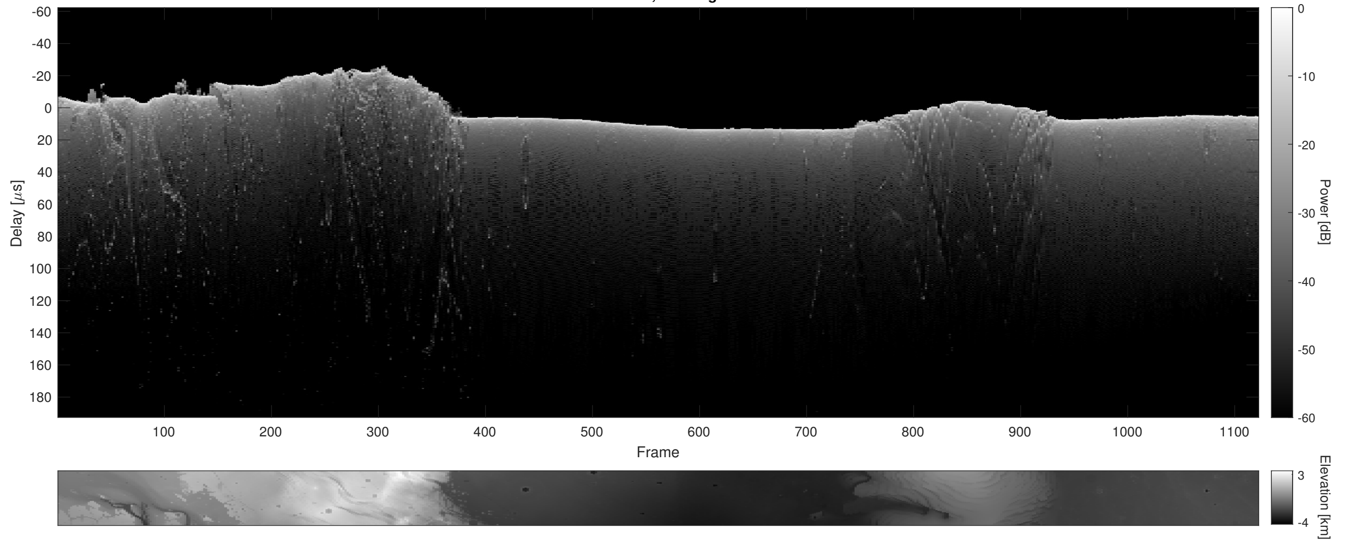
Orbit 12022, Cluttergram
