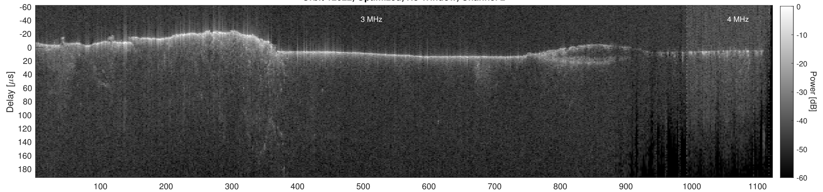
Orbit 12022, Cluttergram
