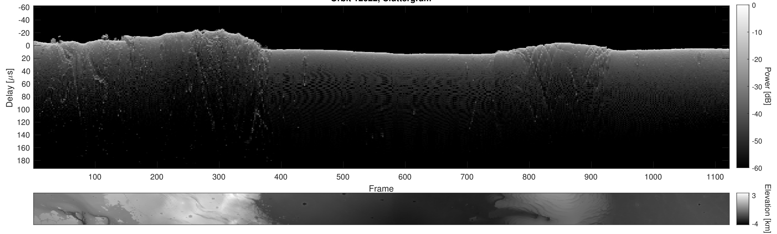
Orbit 12022, Cluttergram
