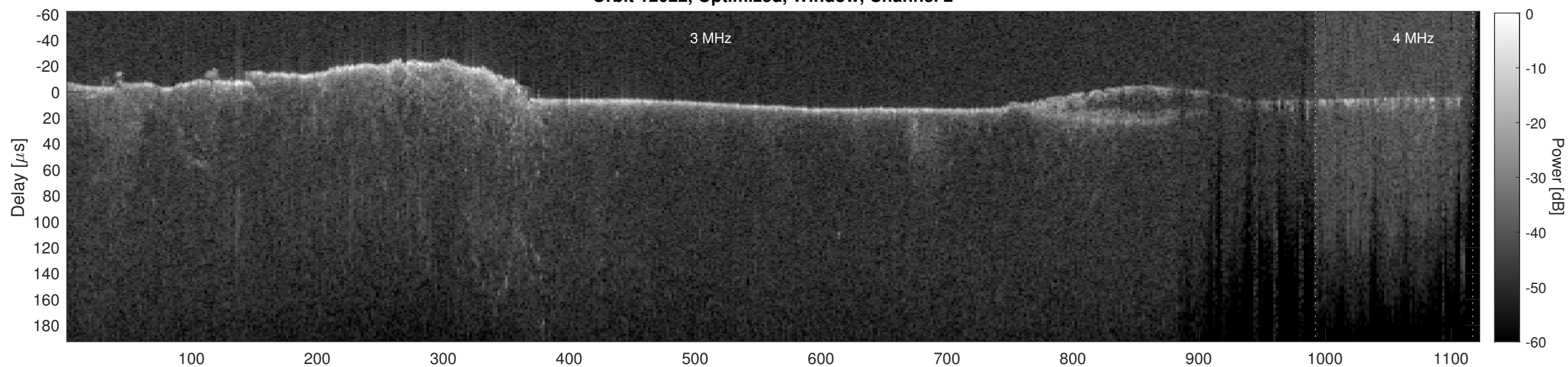
Orbit 12022, Cluttergram
