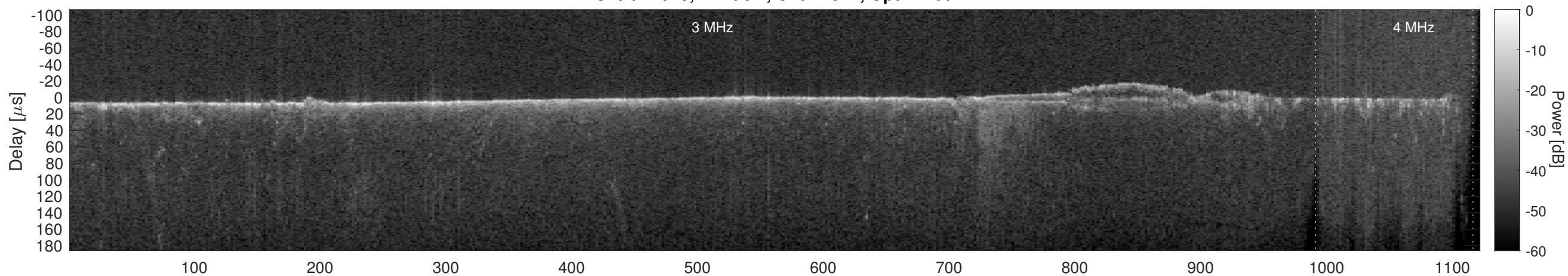
Orbit 12023, Cluttergram
