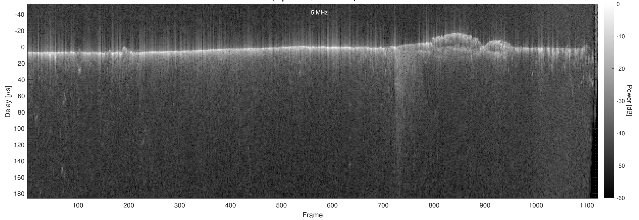
Orbit 12023, Optimized, No Window, Channel 2
