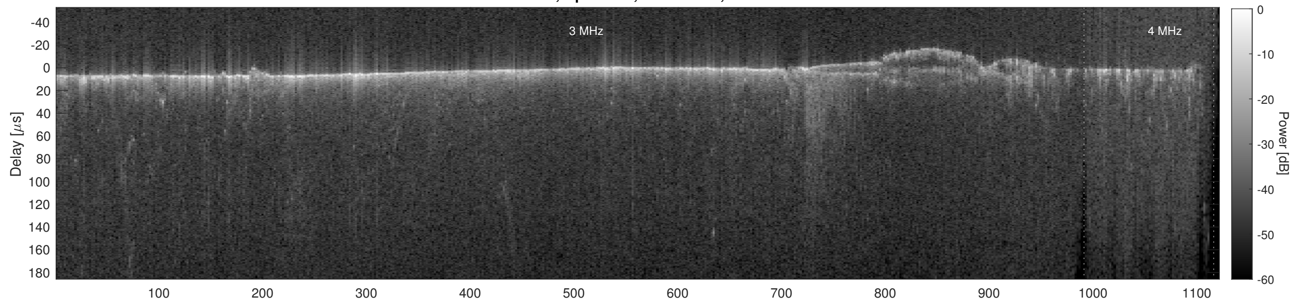
Orbit 12023, Cluttergram
