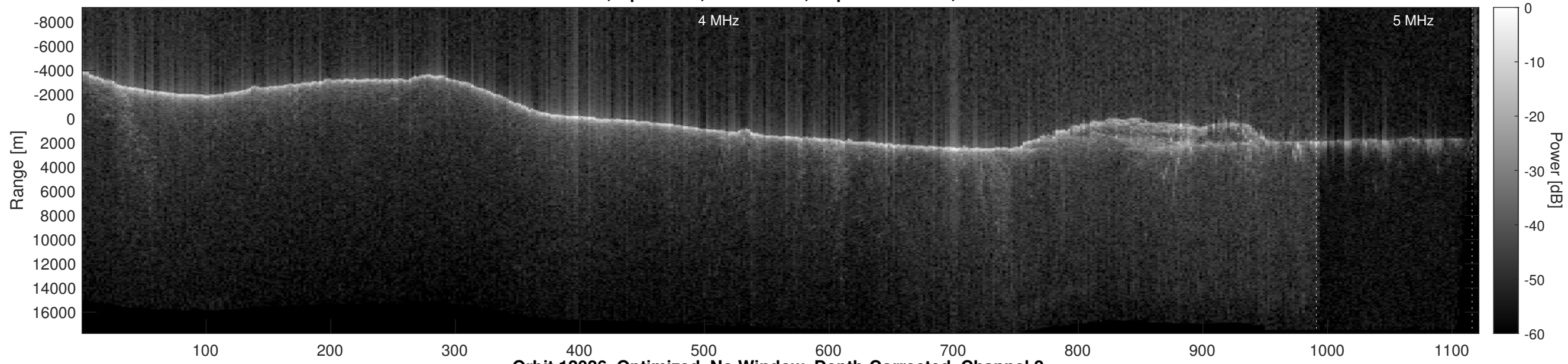
Orbit 12026, Optimized, No Window, Depth-Corrected, Channel 2
