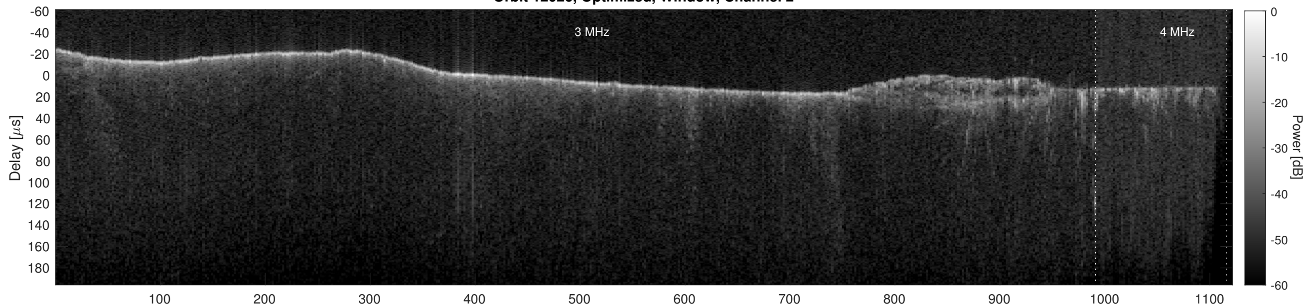
Orbit 12026, Cluttergram
