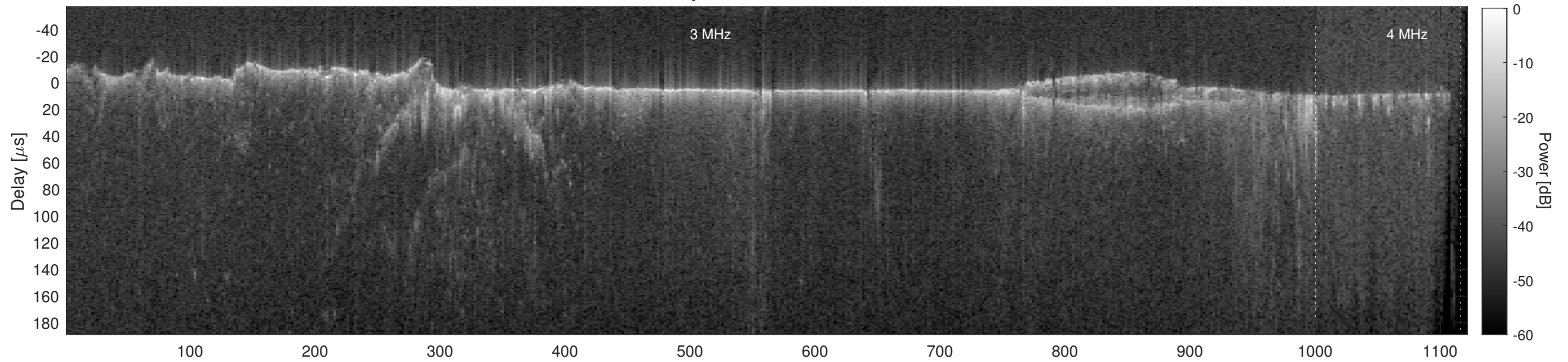
Orbit 12028, Cluttergram
