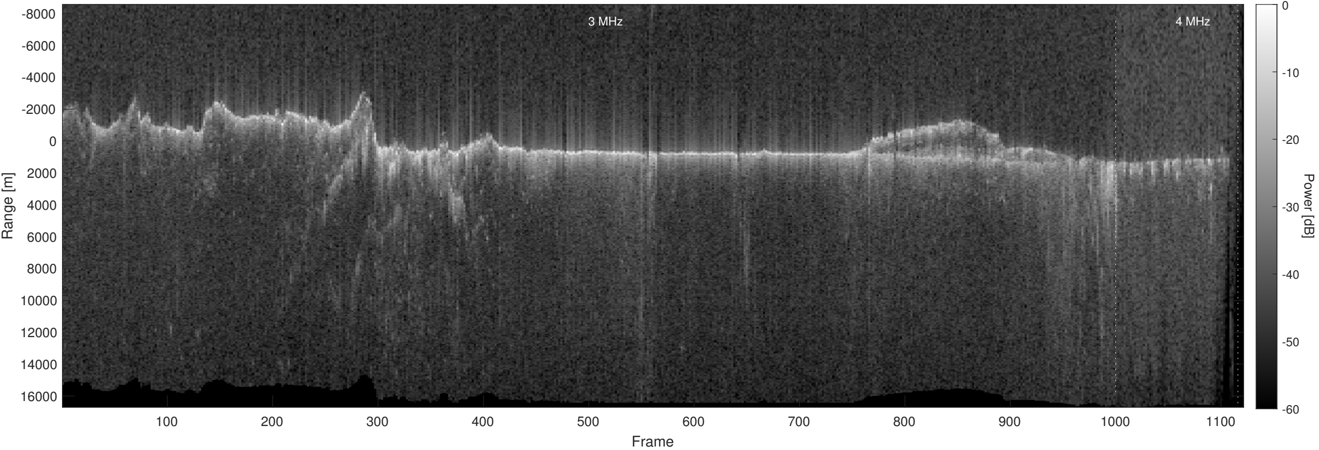
Orbit 12028, Optimized, No Window, Depth-Corrected, Channel 2
