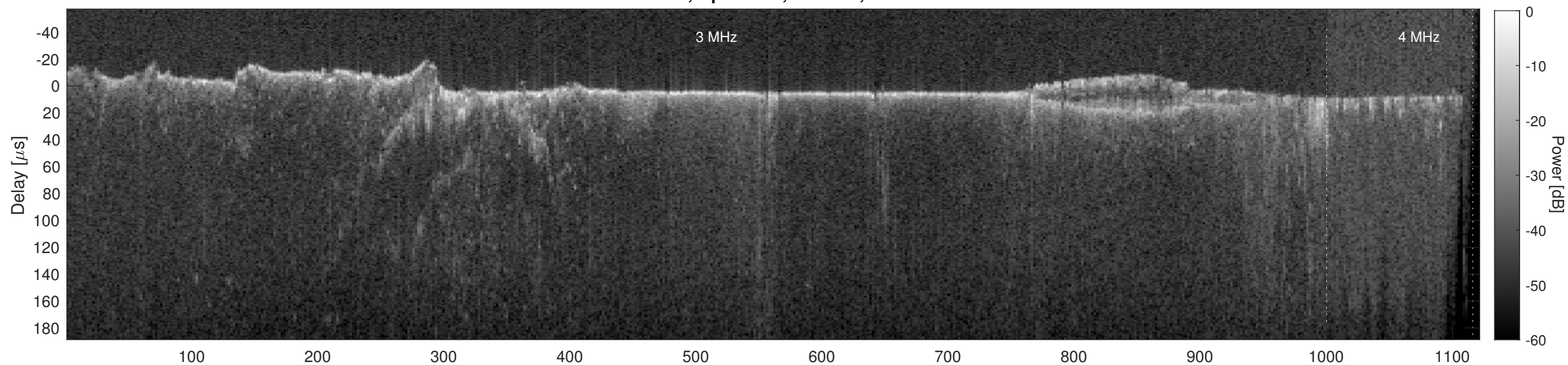
Orbit 12028, Cluttergram
