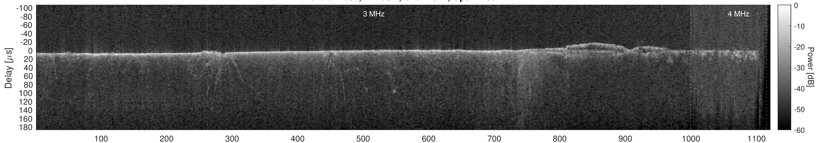
Orbit 12030, Cluttergram
