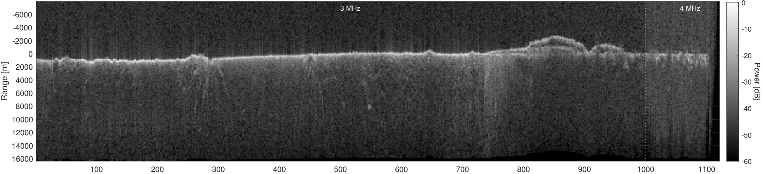
Orbit 12030, Depth-Corrected Cluttergram
