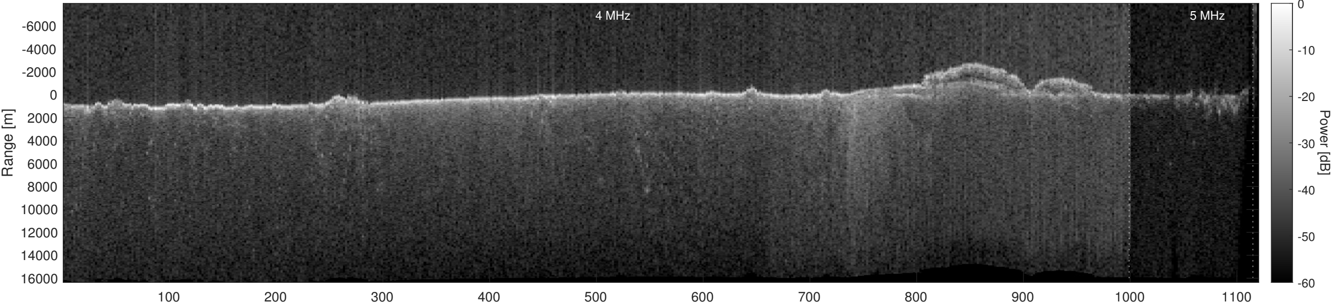
Orbit 12030, Optimized, Window, Depth-Corrected, Channel 2
