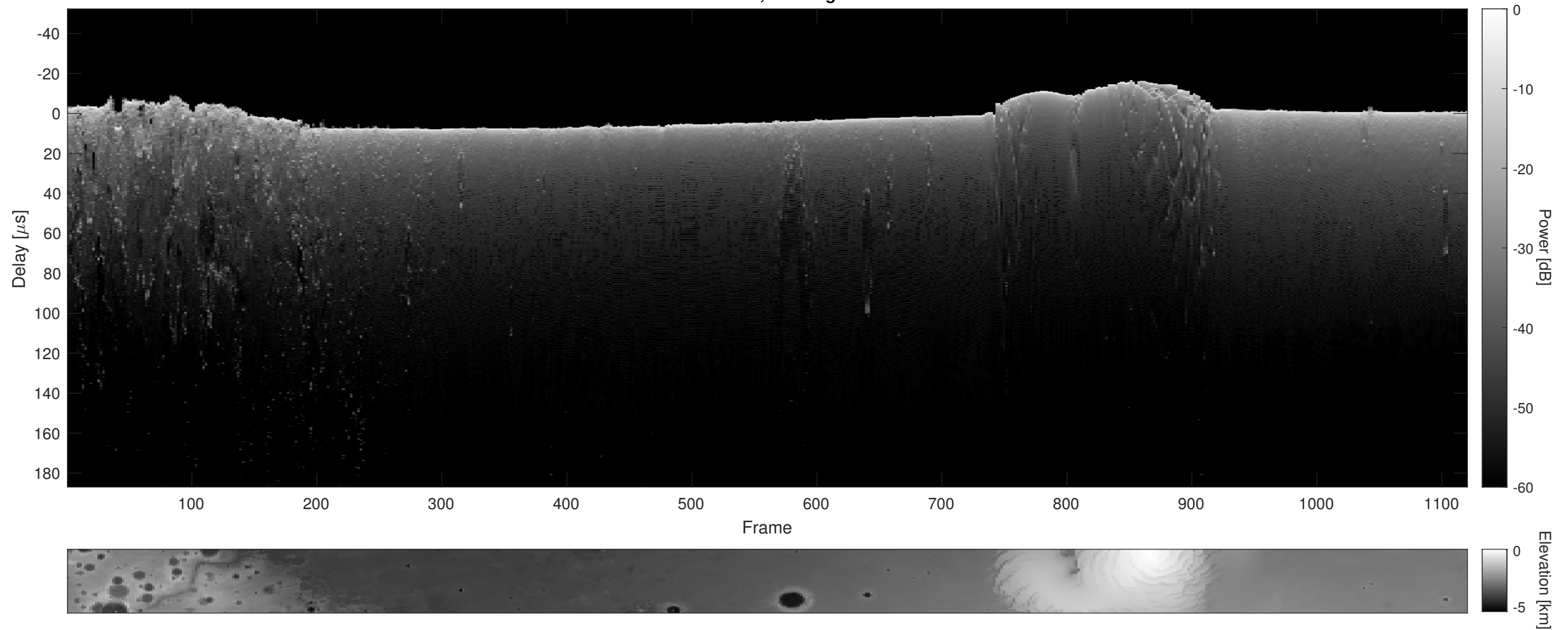
Orbit 12032, Cluttergram
