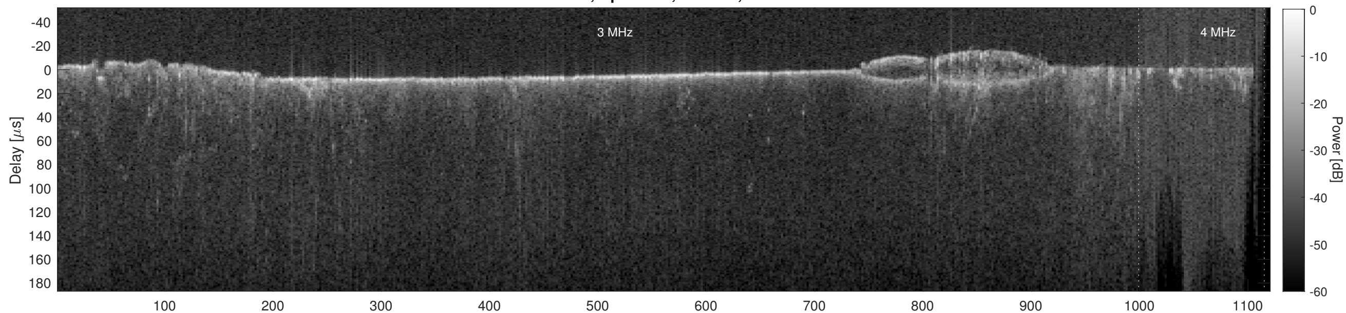
Orbit 12032, Cluttergram
