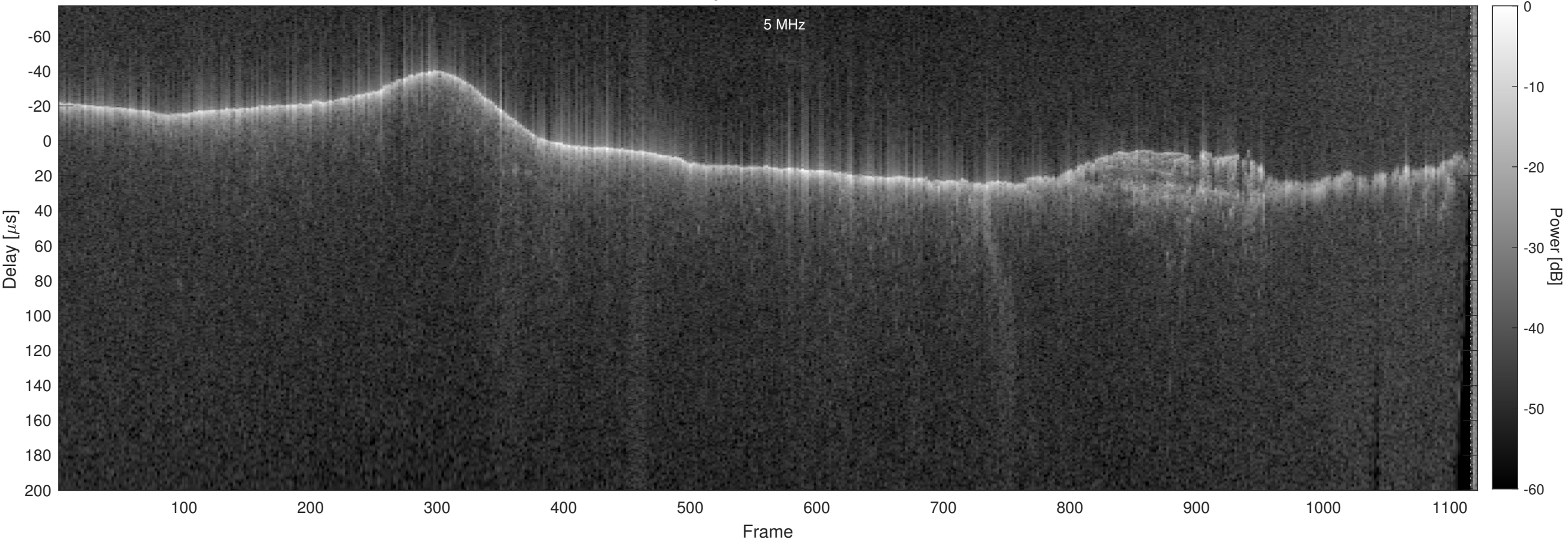
Orbit 12033, Chapman, No Window, Channel 2
