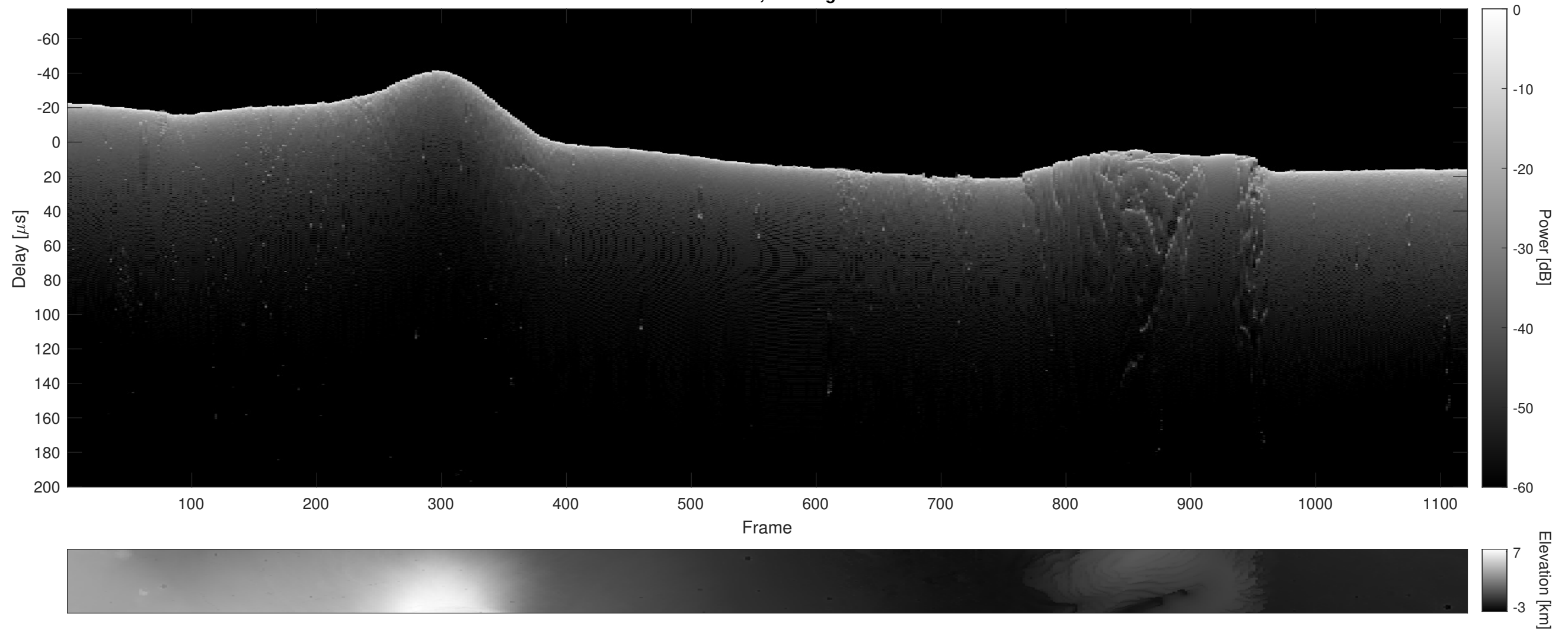
Orbit 12033, Cluttergram
