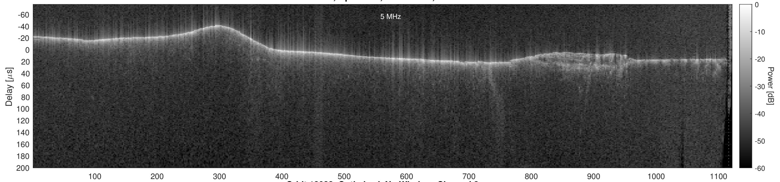
Orbit 12033, Optimized, No Window, Channel 2
