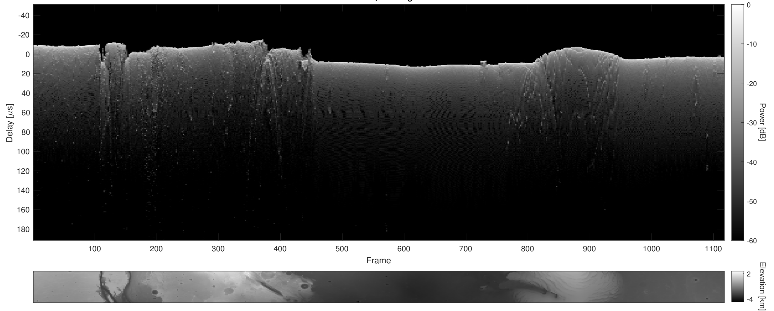
Orbit 12036, Cluttergram
