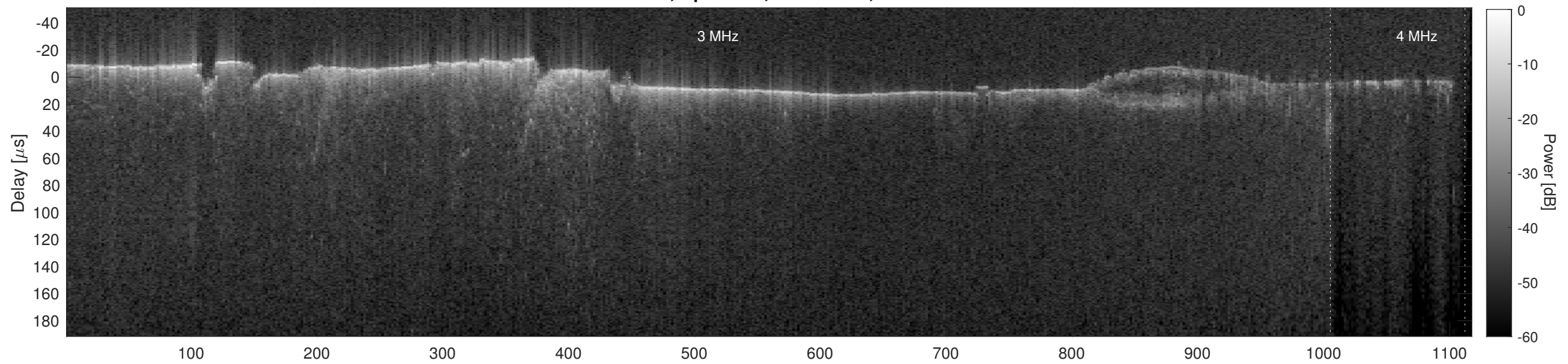
Orbit 12036, Cluttergram
